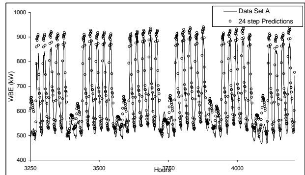
Figure 5: Predicted whole building electricity (WBE) consumption compared with data.
