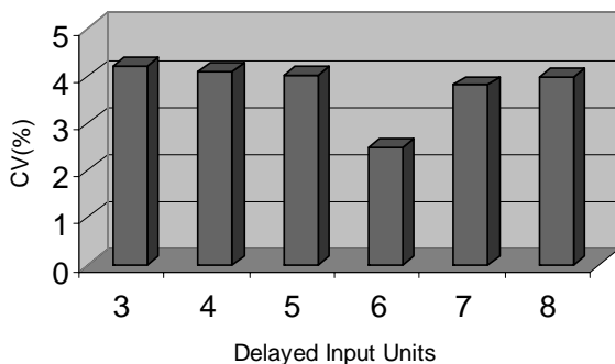
Figure 4: Coefficient of variation vs. delayed input units.
