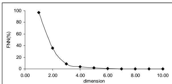
Figure 2: The percentage of global false nearest neighbors.
