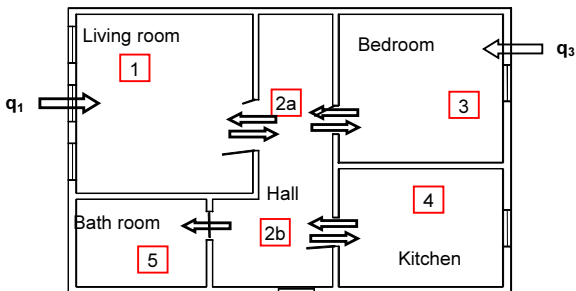
Figure 1. Plan of the test house used in the experiments
