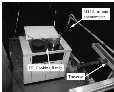
Figure 3. Detail of experimental conditions
