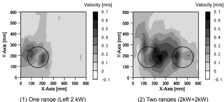
Figure 5. Air flow velocity of updraft (Horizontal section at 800mm, without hood)
