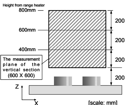
(2) Y-axis section
