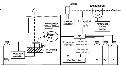
Figure 4. Outline of experiment
