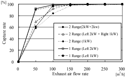
Figure 10. Results of capture ratio (Hood height form the Range is 400mm)
