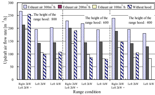
Figure 7. Results of updraft air flow rate
