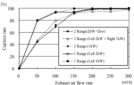
Figure 9. Results of capture ratio (Hood height form the Range is 600mm)
